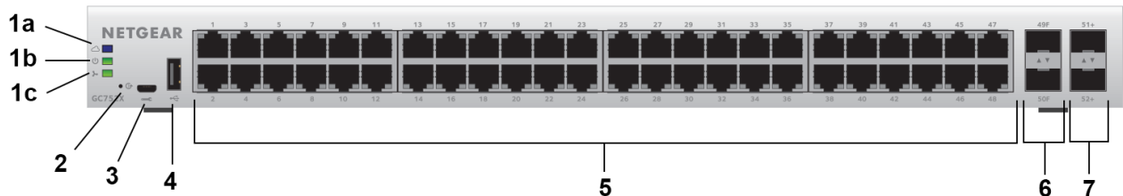
Figure 3. Front panel model GC752X
