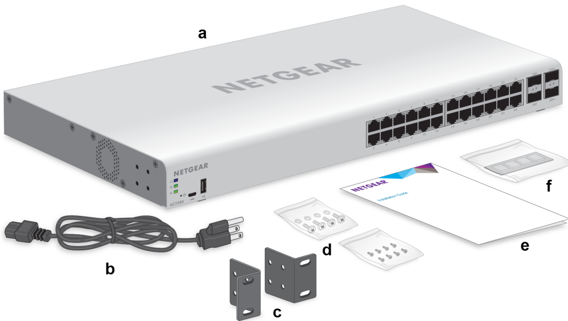
Figure 7. Switch package contents
