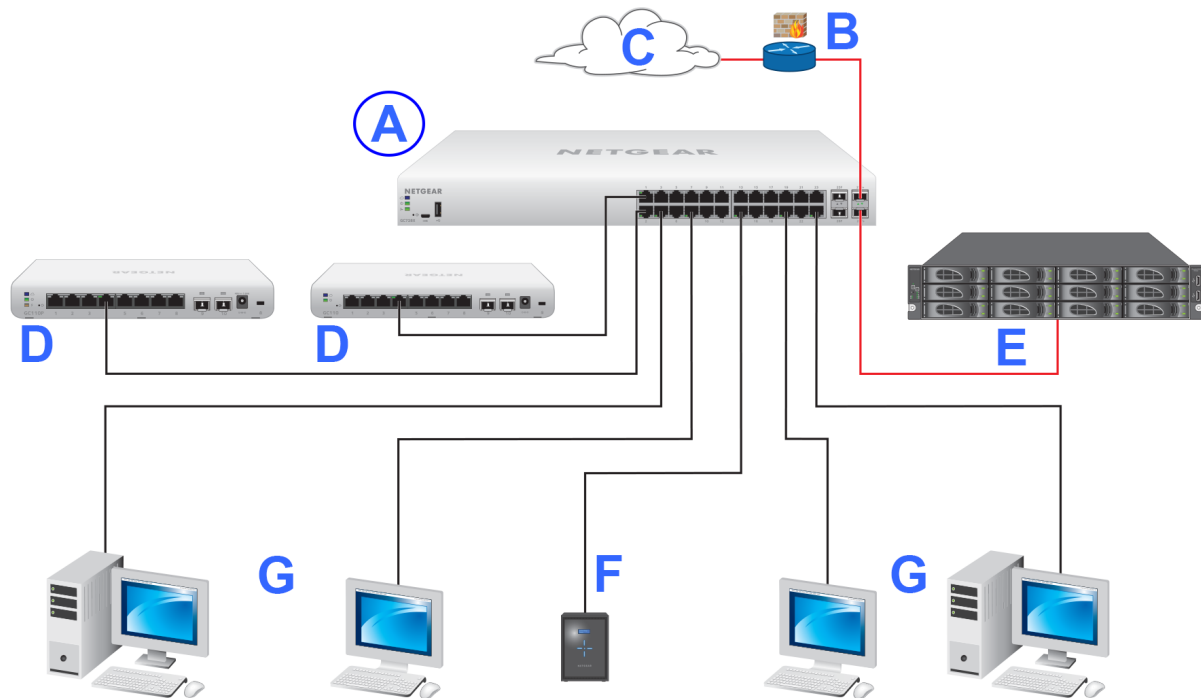
Figure 8. Sample aggregation switching
